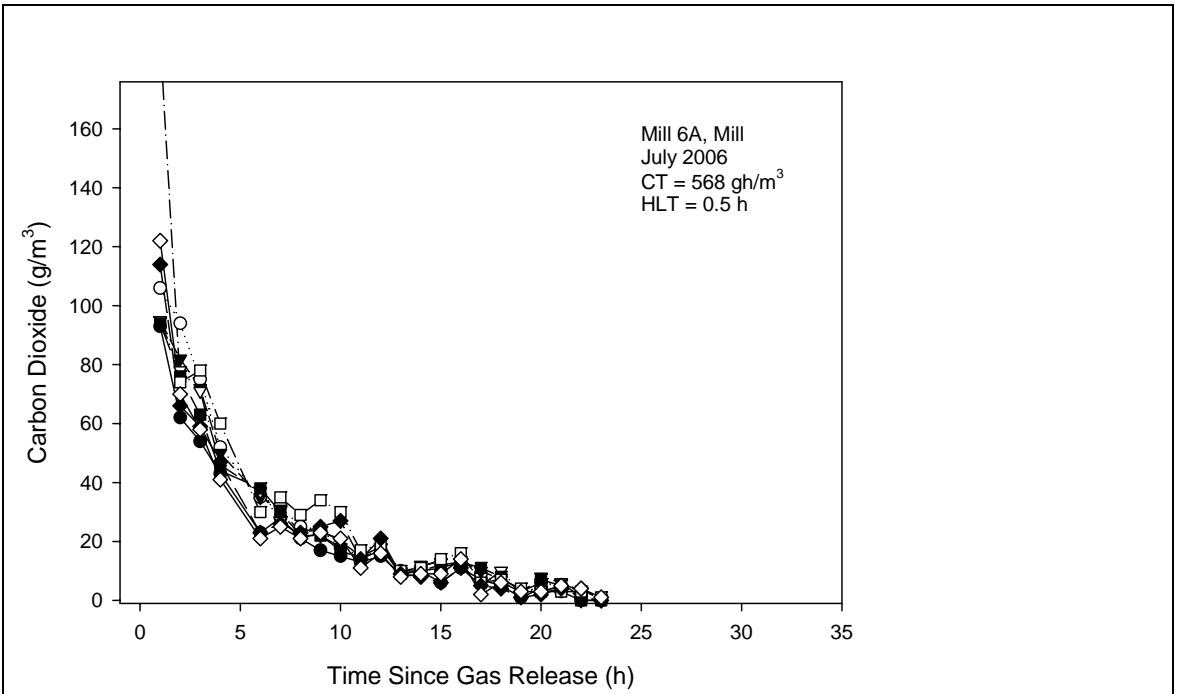
Figure 29. Concentrations of carbon dioxide in Mill 6A (Mill) in July 2005.
