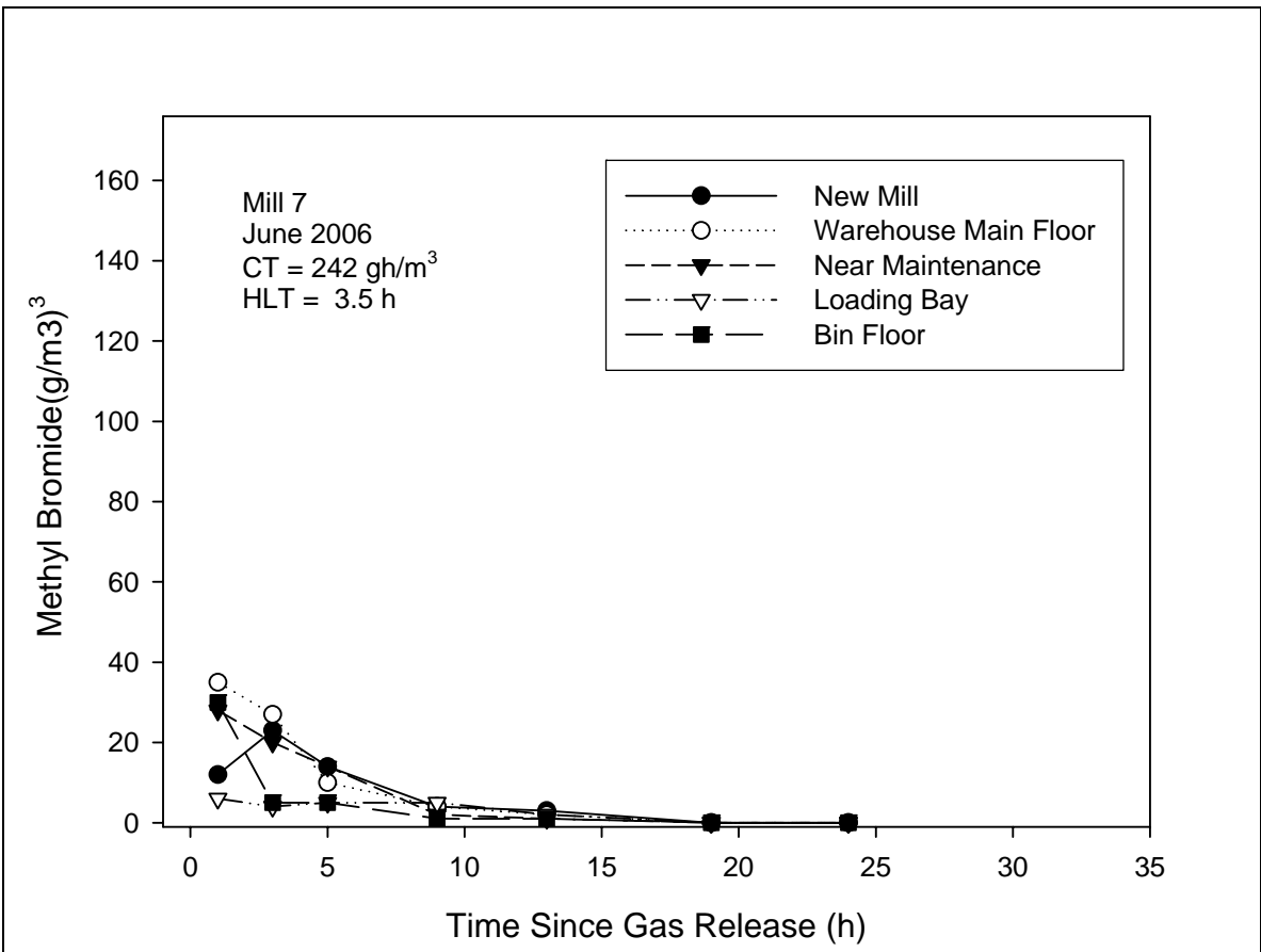
Figure 30. Concentrations of methyl bromide in Mill 7 in June 2006.
