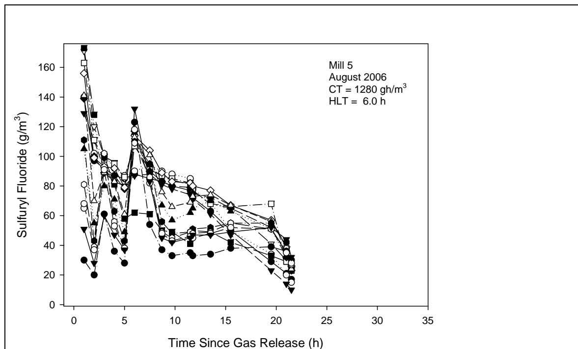
Figure 23. Concentrations of sulfuryl fluoride in Mill 5 in August 2006 .
