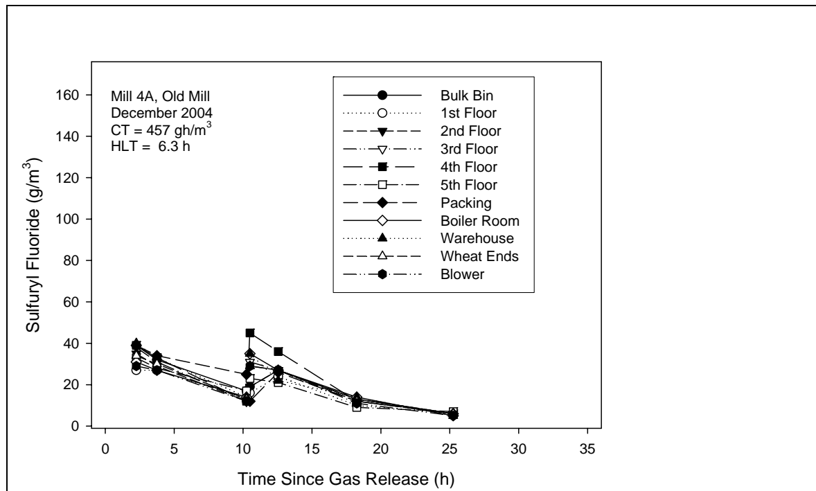
Figure 19. Concentrations of sulfuryl fluoride in Mill 4A (Old Mill) in December 2004.
