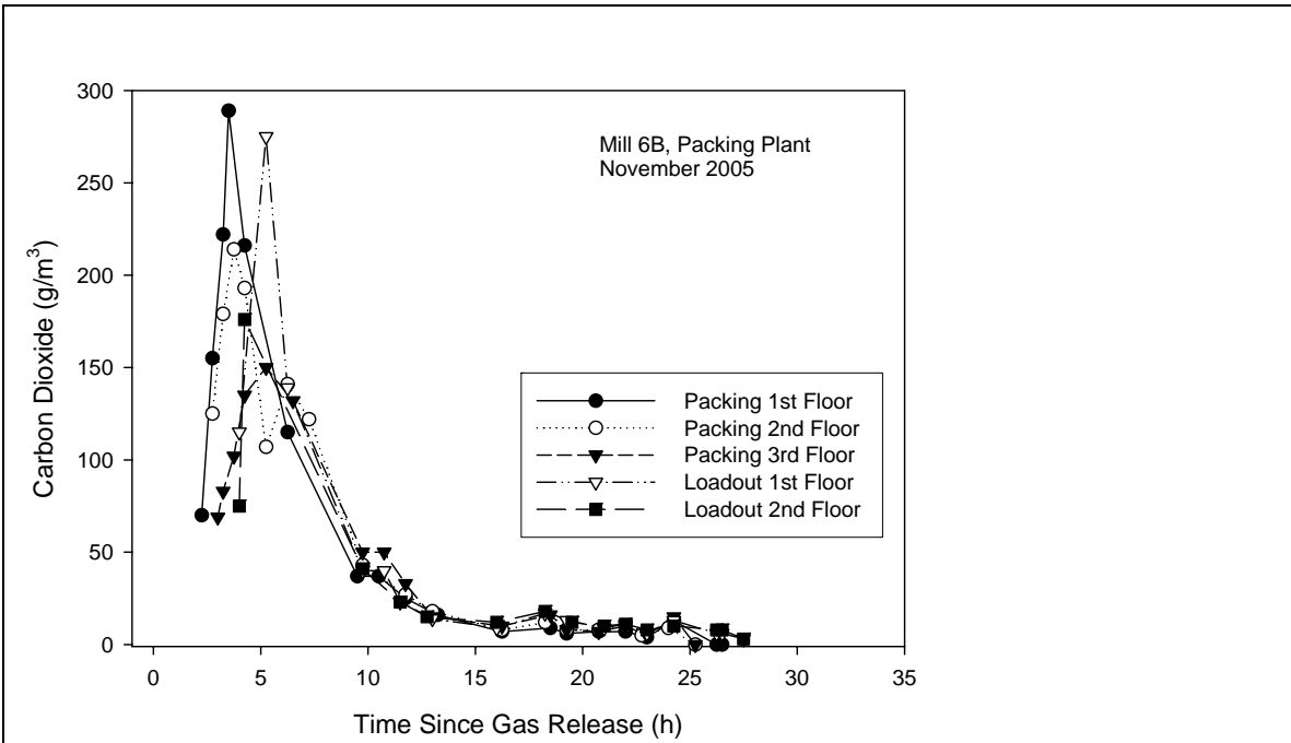
Figure 28. Concentrations of carbon dioxide in Mill 6B (Packing Plant) in November 2005.
