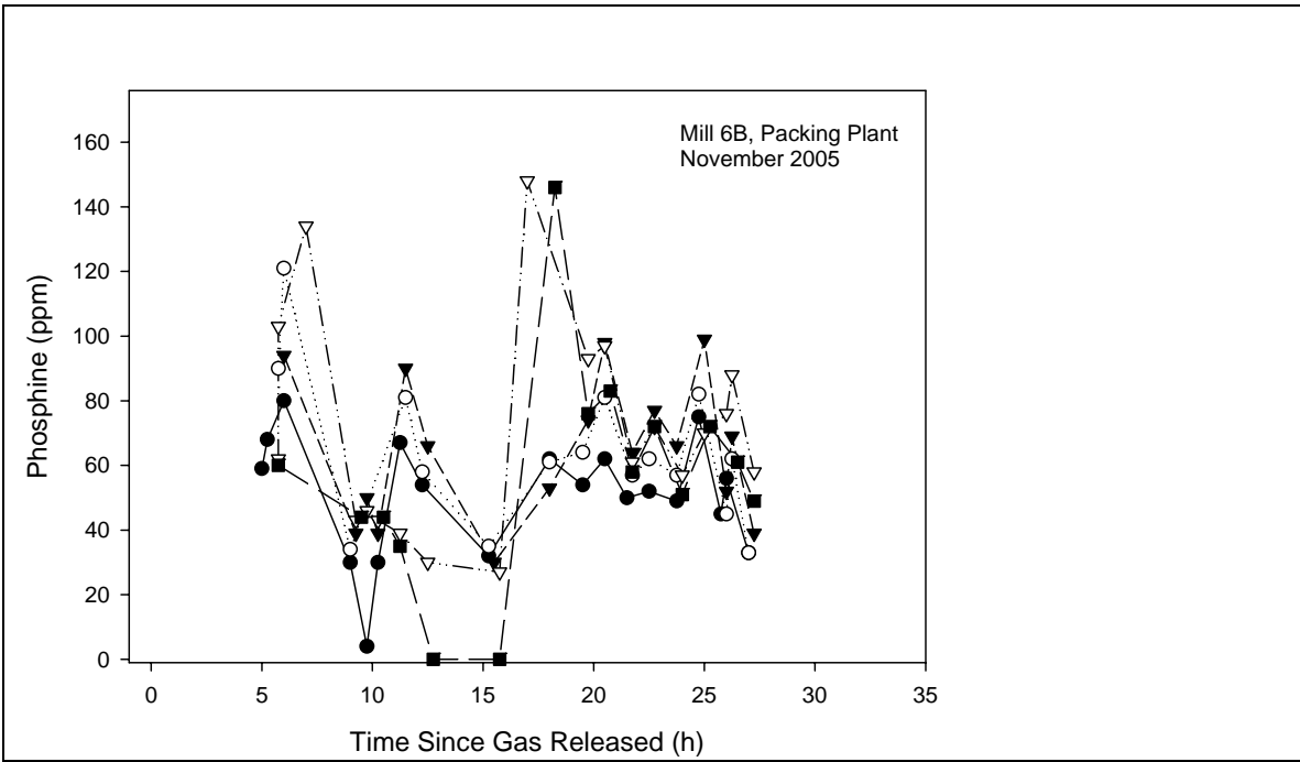
Figure 27. Concentrations of phosphine in Mill 6B (Packing Plant) in November 2005.
