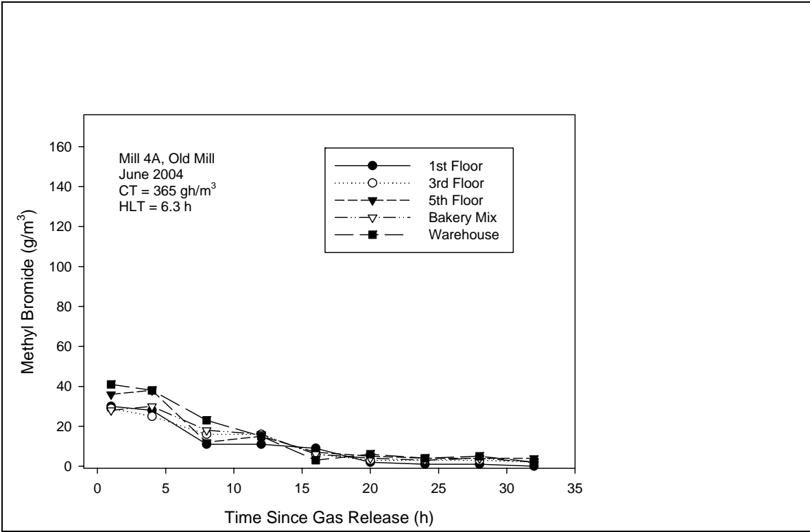
Figure 15. Concentrations of methyl bromide in Mill 4A (Old Mill) in June 2004.
