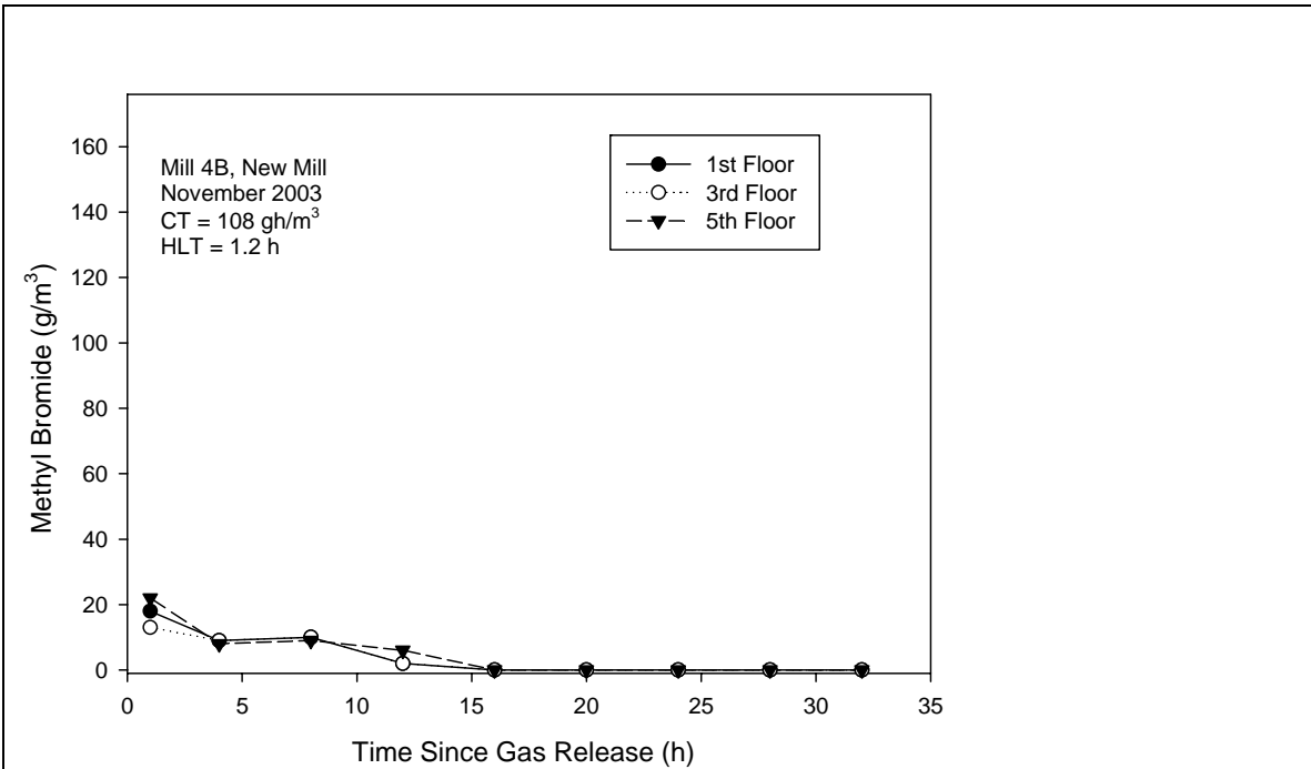
Figure 14. Concentrations of methyl bromide in Mill 4B (New Mill) in November 2003.
