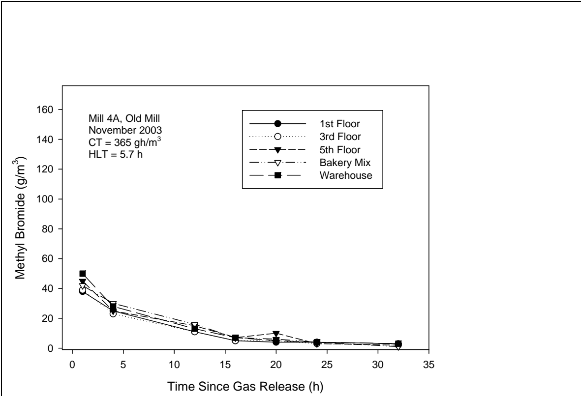
Figure 13. Concentrations of methyl bromide in Mill 4A (Old Mill) in November 2003.
