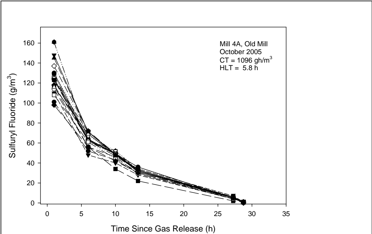
Figure 21. Concentrations of sulfuryl fluoride in Mill 4A (Old Mill) in October 2005.
