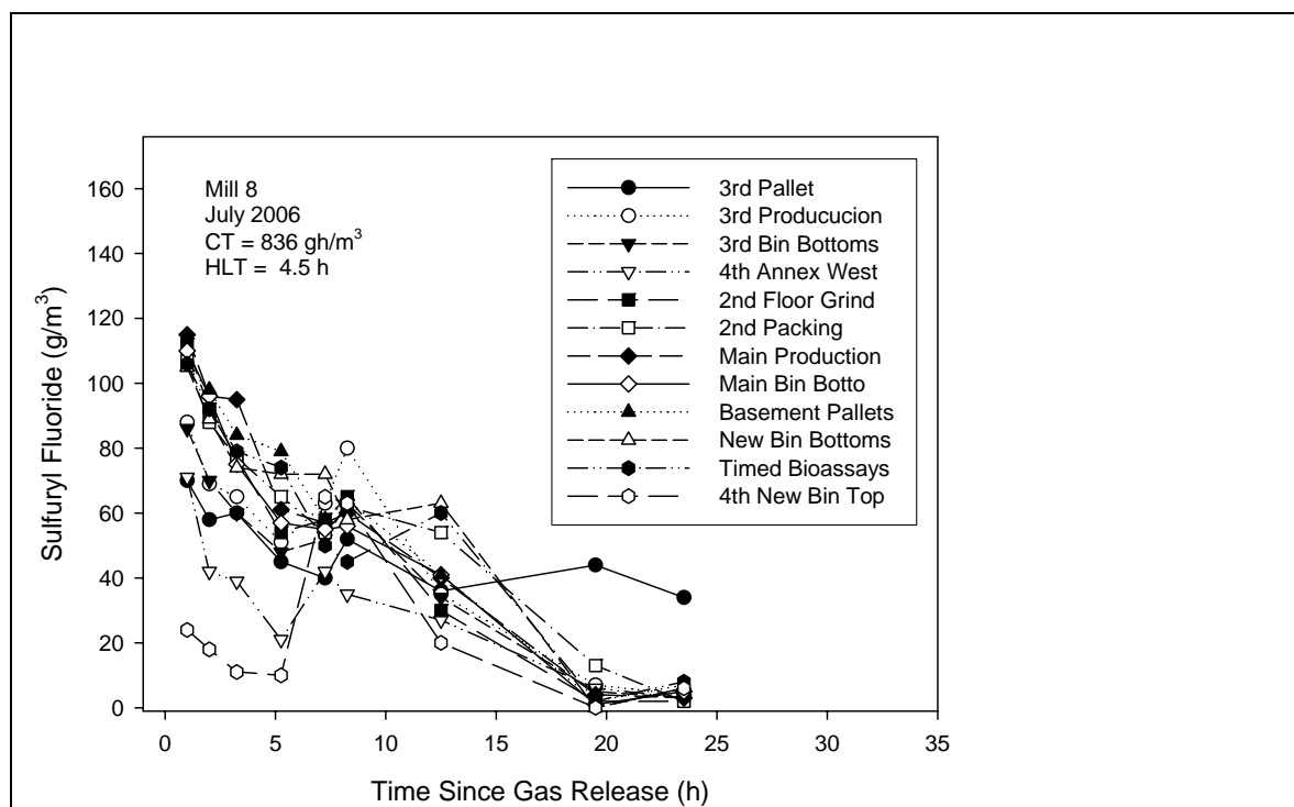
Figure 24. Concentrations of sulfuryl fluoride in Mill 8 in July 2006.
