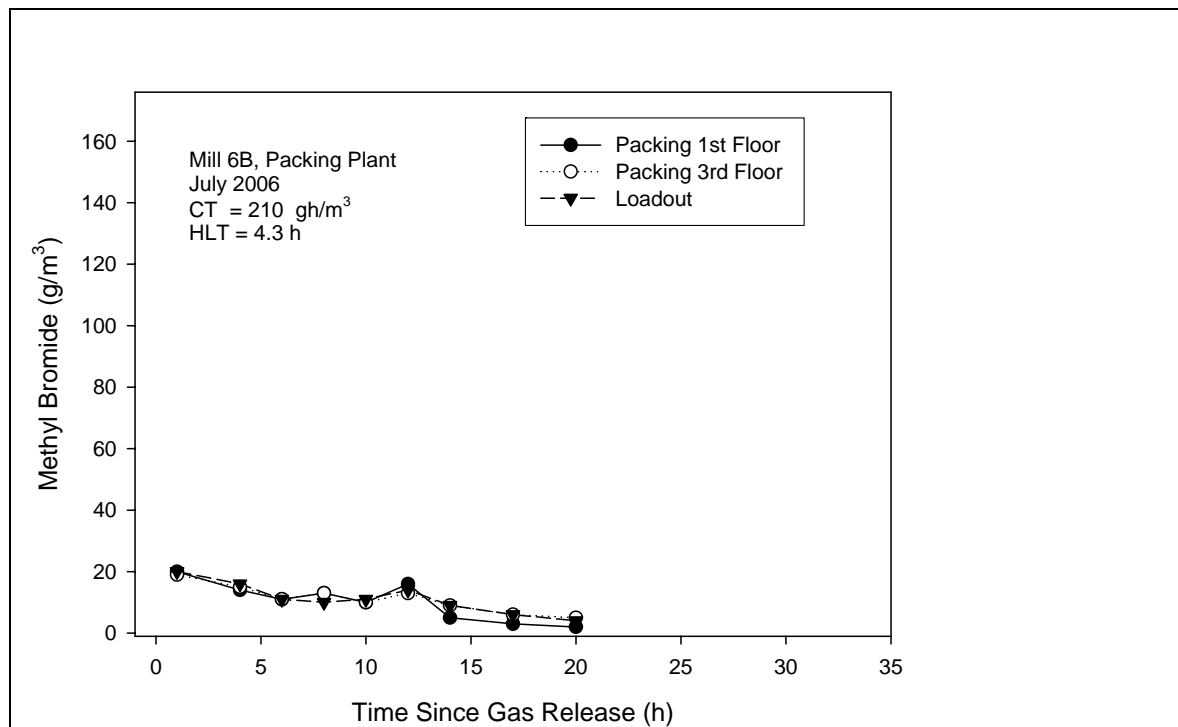
Figure 26. Concentrations of methyl bromide in Mill 6B (Packing Plant) in July 2006 .
