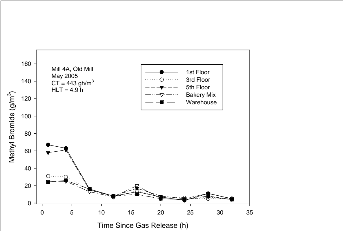
Figure 17. Concentrations of methyl bromide in Mill 4A (Old Mill) in May 2005.
