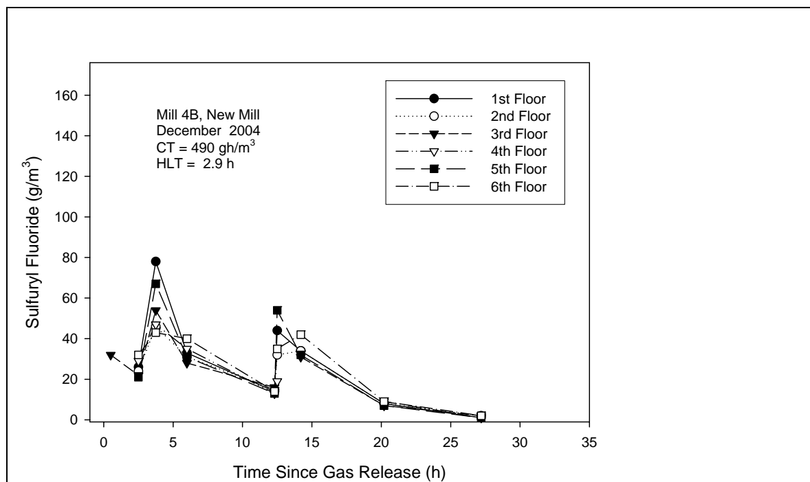
Figure 20. Concentrations of sulfuryl fluoride in Mill 4B (New Mill) in December 2004.
