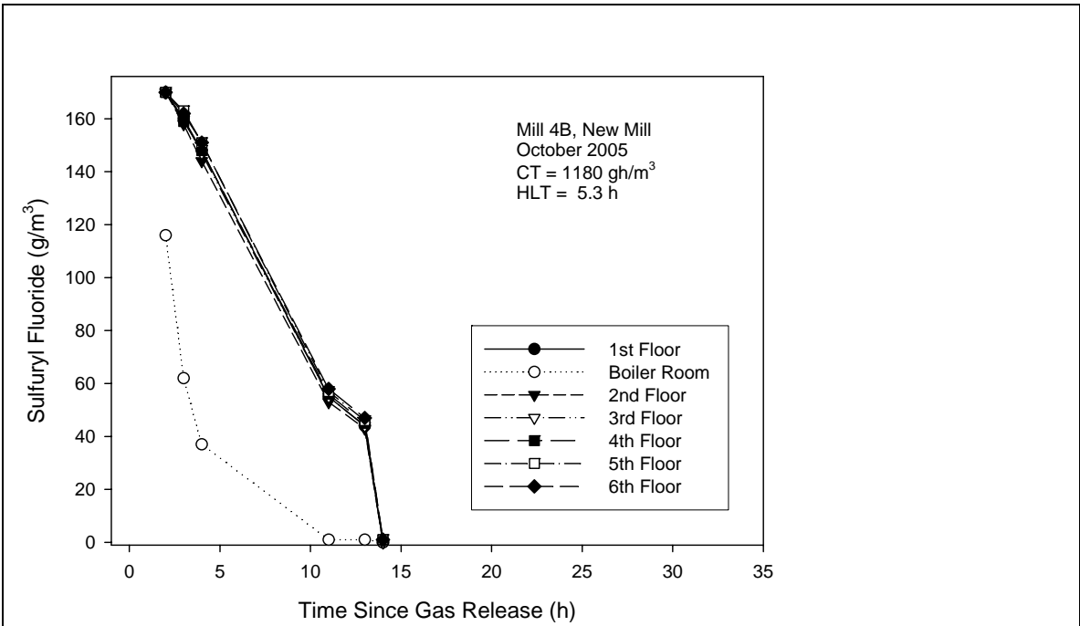
Figure 22. Concentrations of sulfuryl fluoride in Mill 4B (New Mill) in October 2005.
