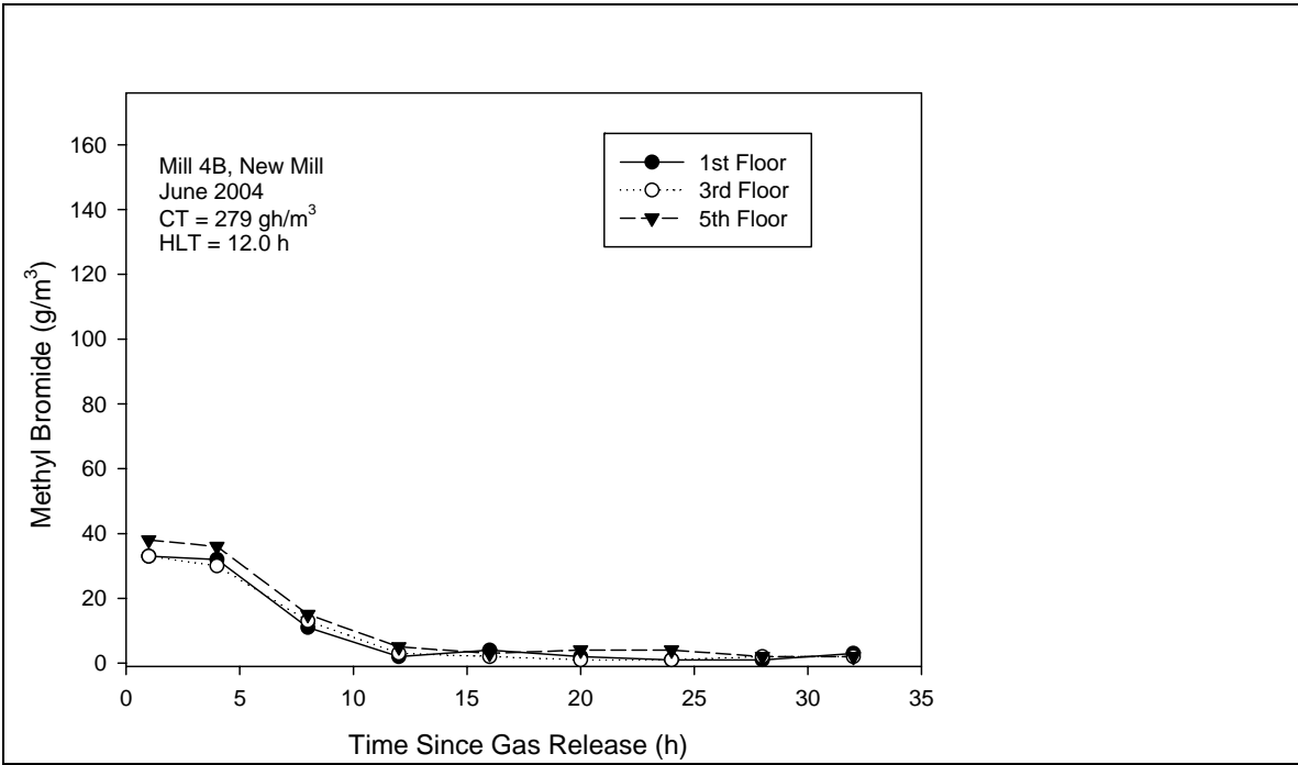
Figure 16. Concentrations of methyl bromide in Mill 4B (New Mill) in June 2004.
