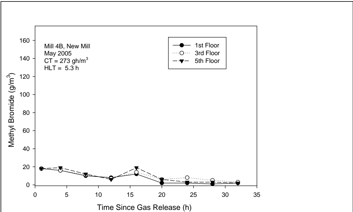
Figure 18. Concentrations of methyl bromide in Mill 4B (New Mill) in May 2005.
