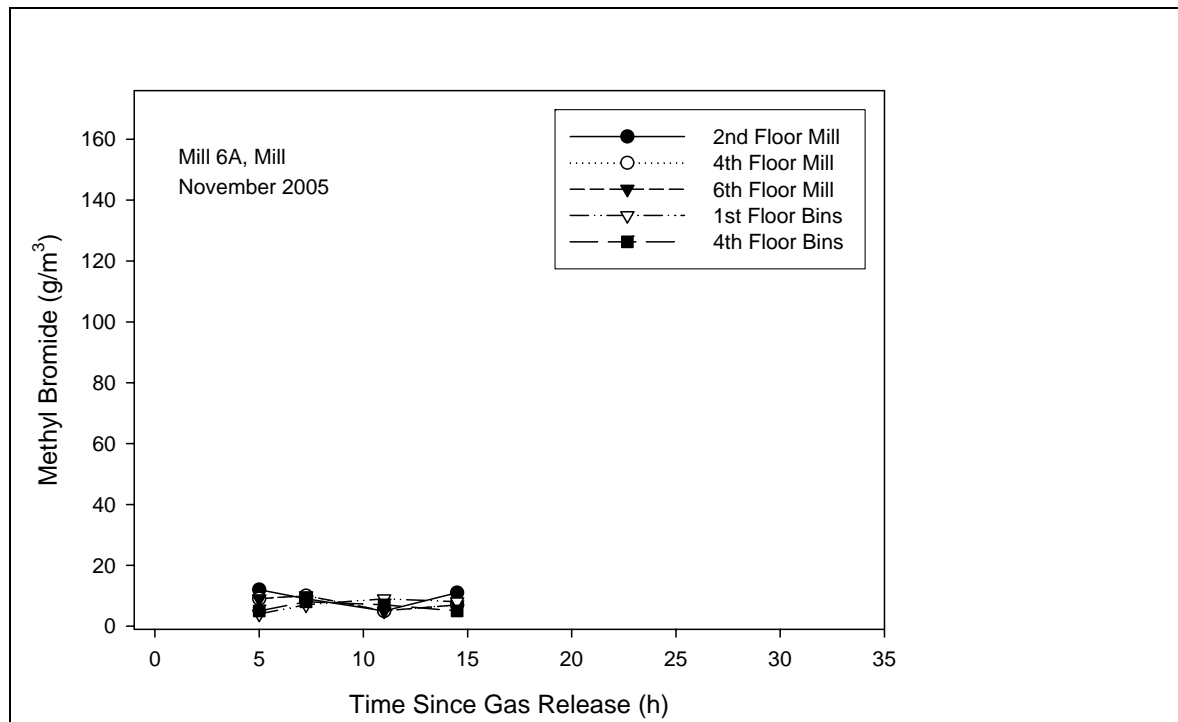
Figure 25. Concentrations of methyl bromide in Mill 6A (Mill) in November 2005 .
